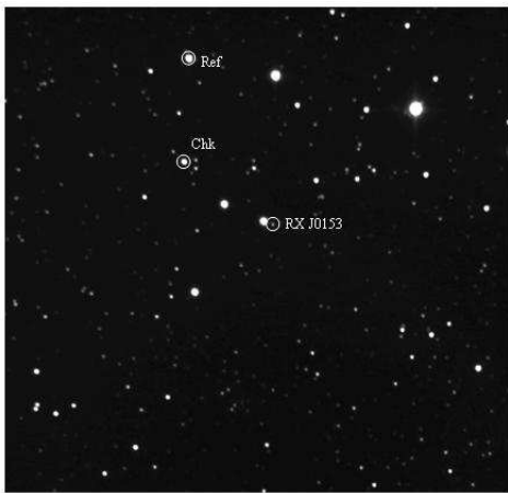
Fig. 1. The field of RX J0153.3+7446. The reference star and check star used for the photometry are indicated. The field shown here is about 12 arcminutes across, North is up and East to the left.
