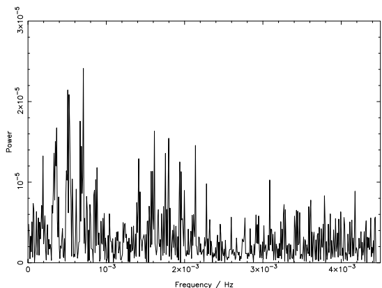
Fig. 5. The power spectrum of the RX J0153.3+7446 ROSAT X-ray lightcurve. Significant power is seen at frequencies of 7.05 \times 10^{-4} Hz (i.e. 1414s) and at 5.06 \times 10^{-4} Hz, corresponding to a period of 1974s.
