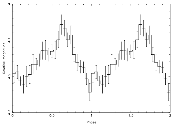
Fig. 4. The optical lightcurve of RX J0153.3+7446, folded at 2333s and binned into 25 phase bins. Magnitudes are relative to TYC 4322-255-1 and the phasing is arbitrary.
